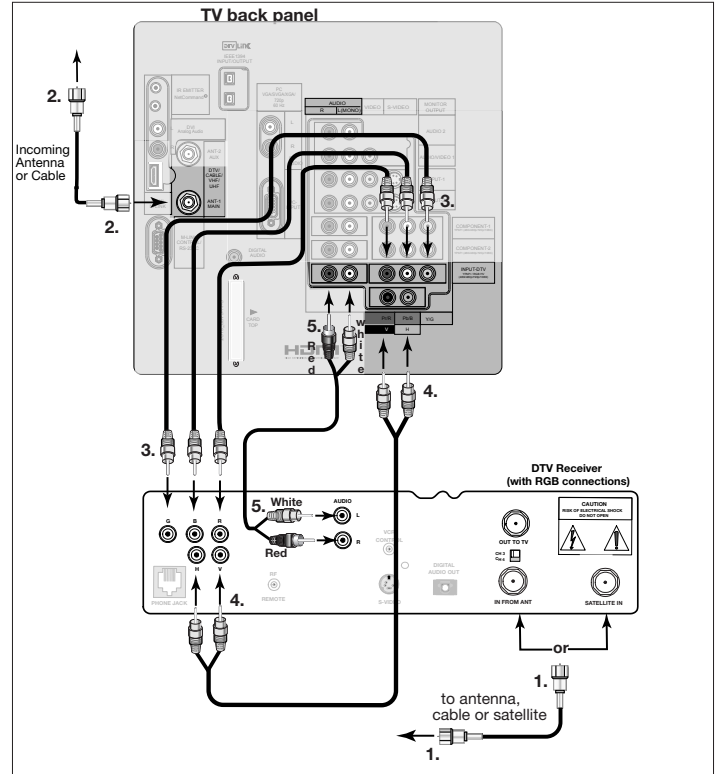
Figure 13. Connecting an External DTV Receiver with RGB Video Connections
