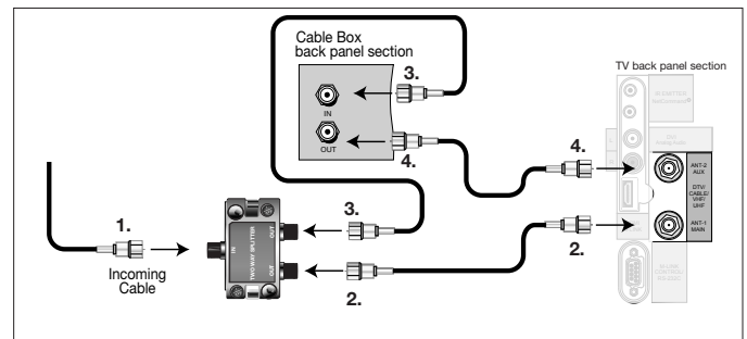
Figure 2. Connecting a Cable Box
